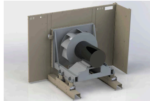
Figure 4: DDP supply fan
