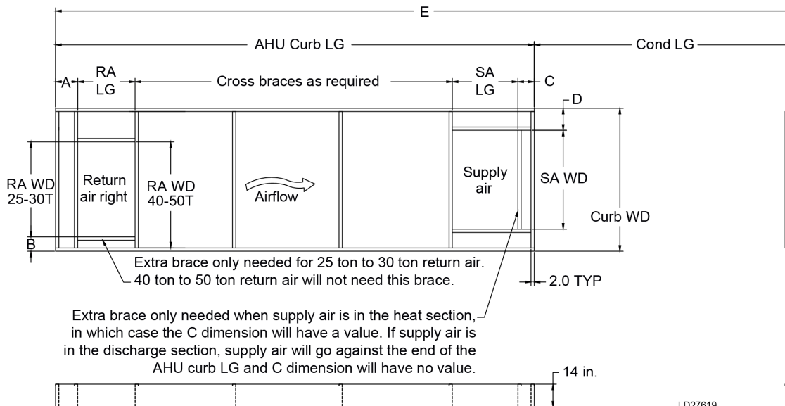
Figure 21: 25 ton to 50 ton roof curbs: right bottom return opening and bottom supply opening without ERW
