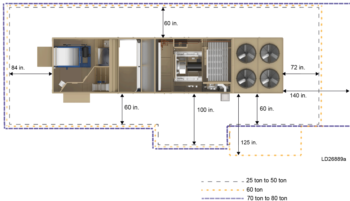
Figure 25: Unit clearances
