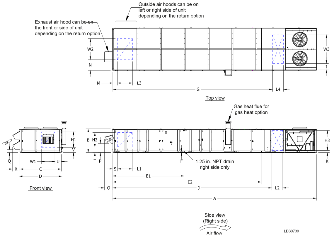
Figure 15: 25 ton to 30 ton dimensional drawing
