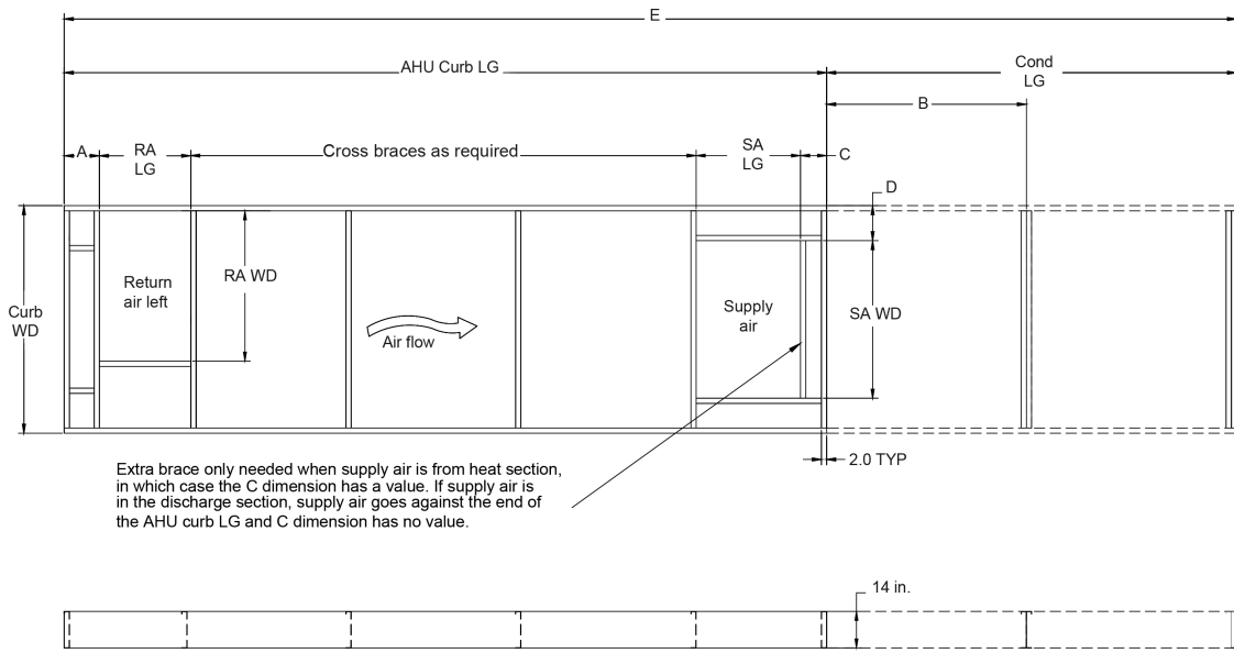
Figure 22: 60 ton to 80 ton roof curbs left bottom return opening and bottom supply opening without ERW
