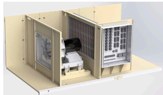
Figure 6: Electric heat
