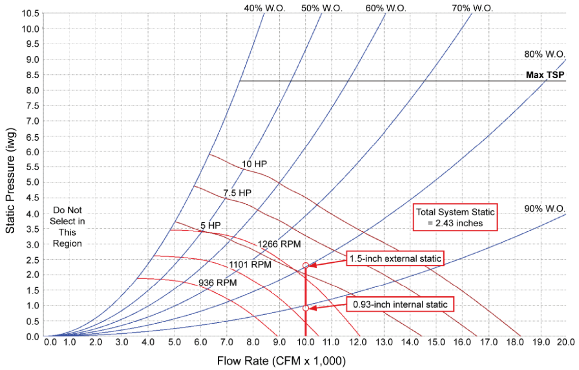
Figure 12: 25 ton unit fan performance
