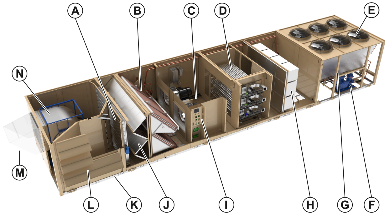
Figure 3: 25 ton to 80 ton packaged rooftop unit cabinet assembly
