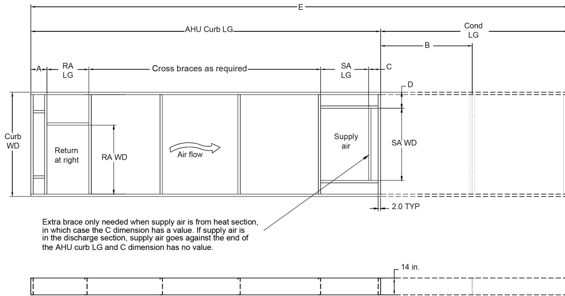
Figure 23: 60 ton to 80 ton roof curbs right bottom return opening and bottom supply opening without ERW
