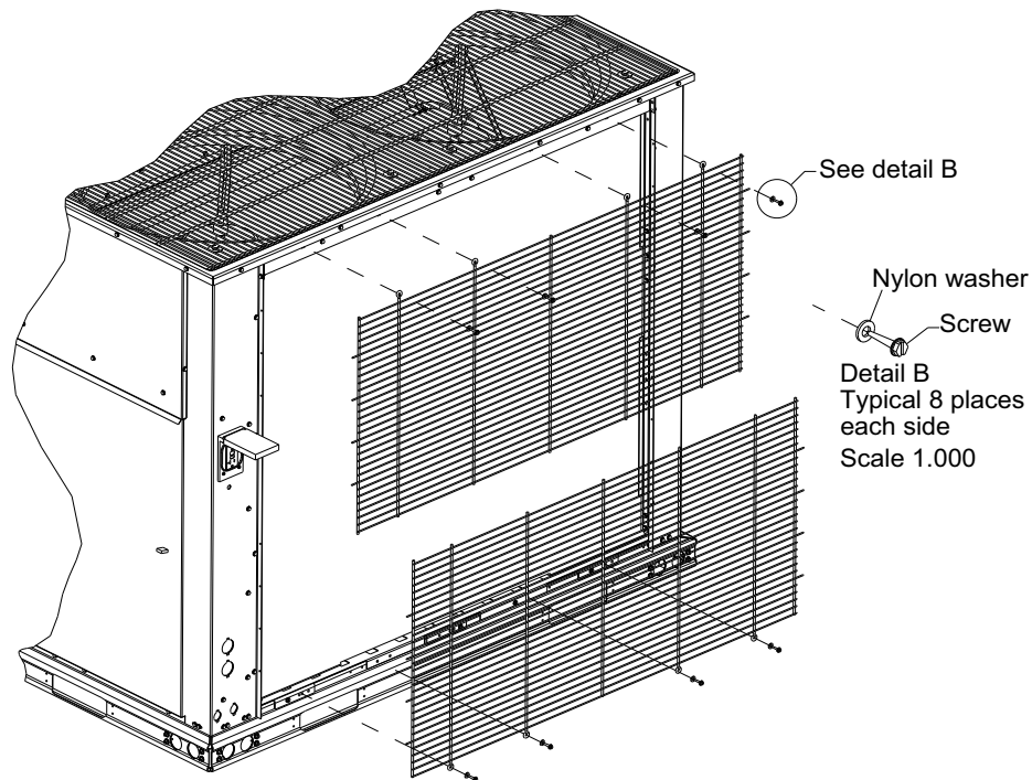
Figure 2: Installing 1CG0404
