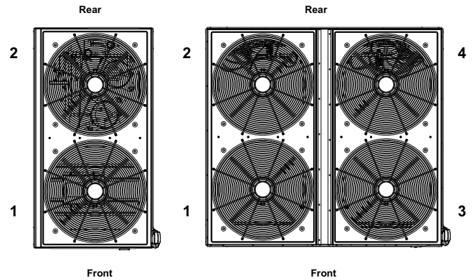
Figure 10: Fan Orientation - Control Box End
