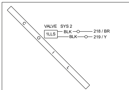
Figure 5: Typical GL120 - 240 liquid line solenoid wiring
