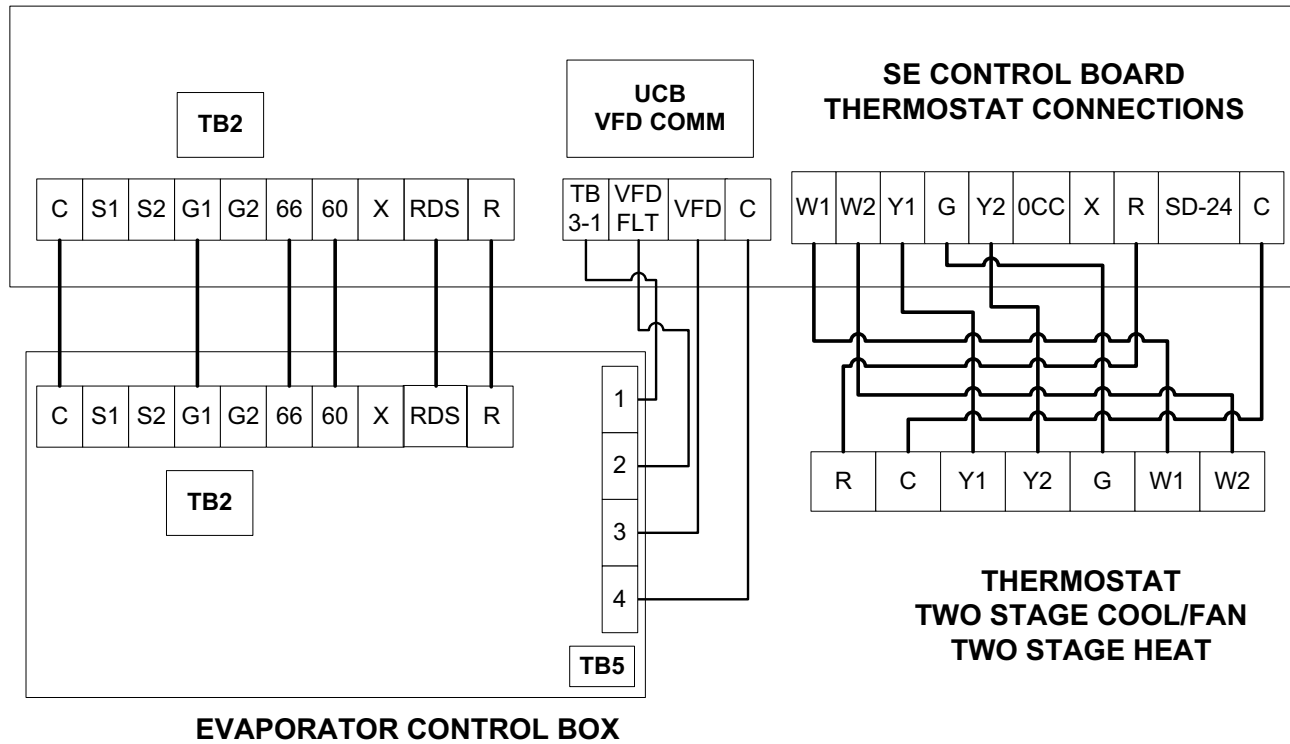
Figure 6: Typical simplified field wiring diagram – GM120 to 240 evaporator with KD120 to 240 condenser
