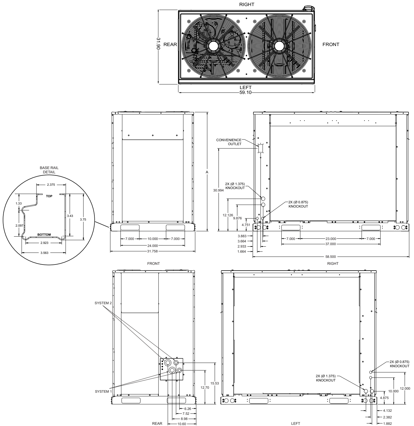
Figure 8: KE090, KC/KD120, and KC/KD150 unit dimensions
