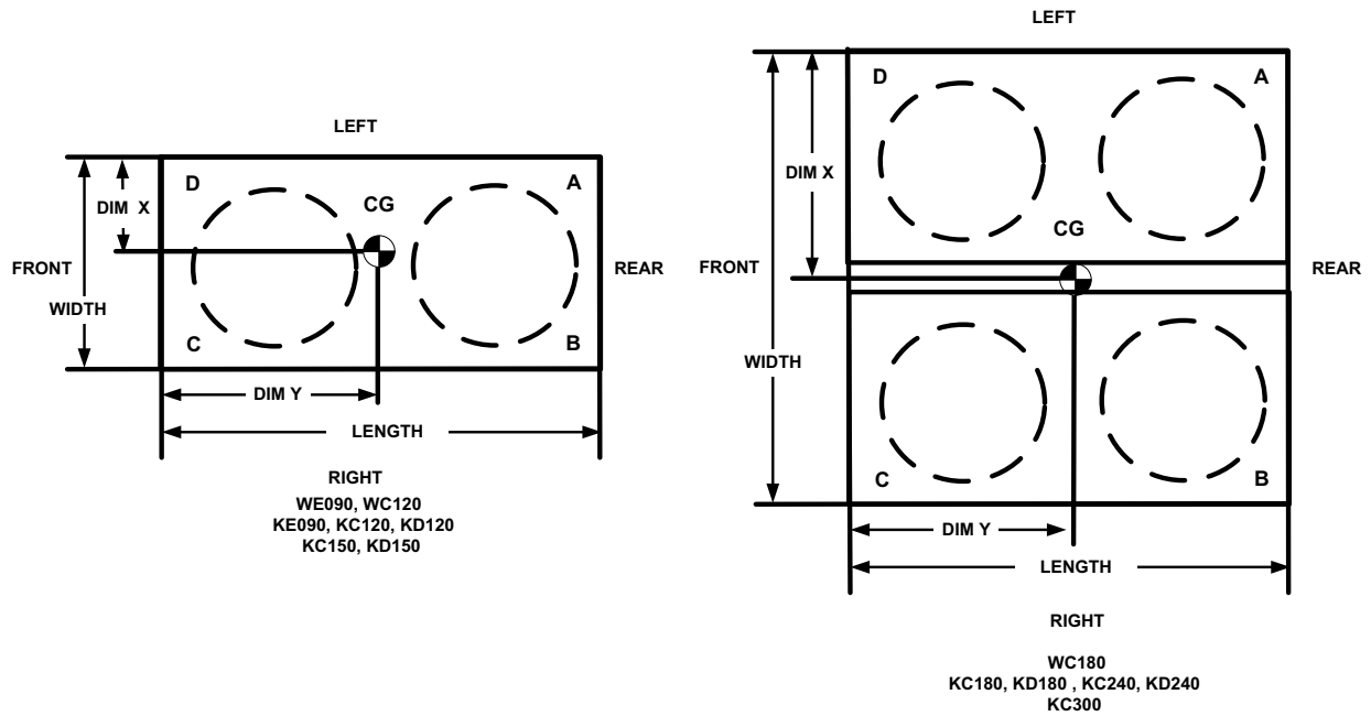
Figure 1: Corner weights and center of gravity
