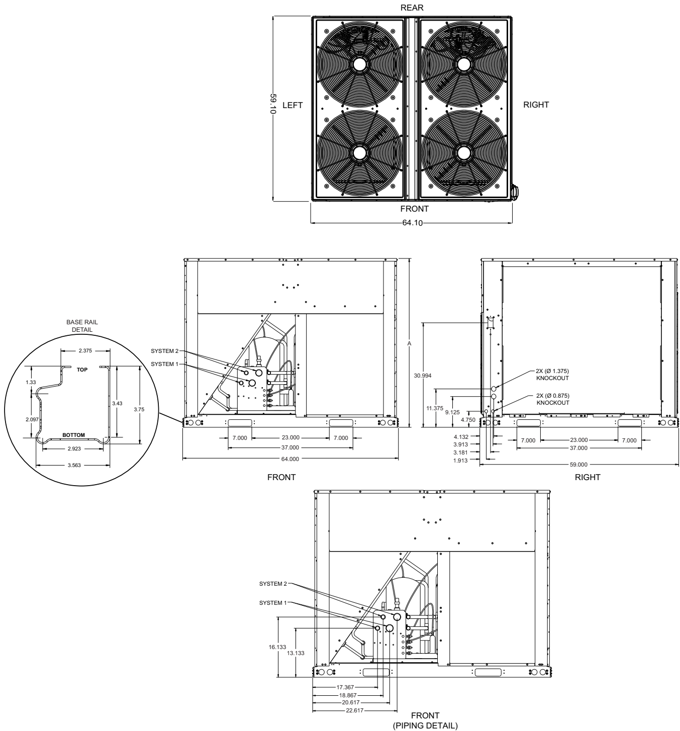
Figure 9: KC/KD180 and KC/KD240 unit dimensions and piping and electrical dimensions
