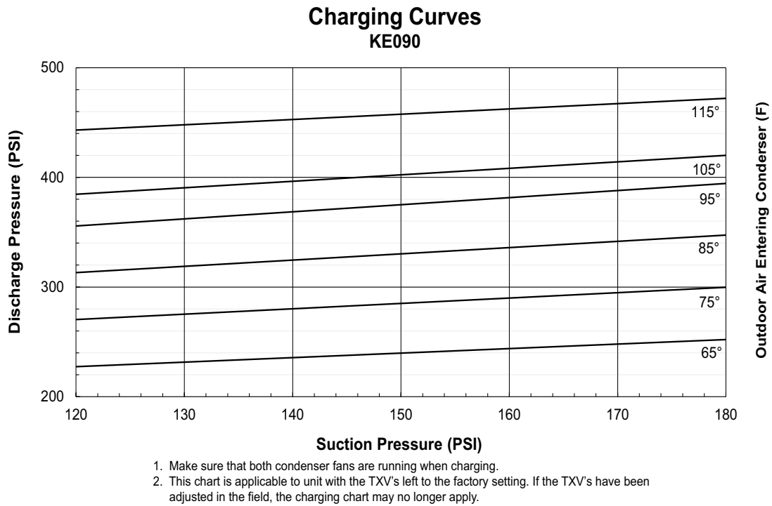
Figure 14: KE090 charging chart
