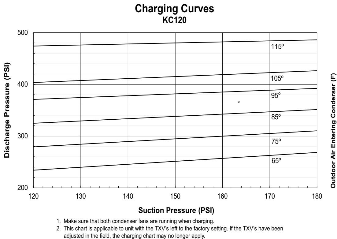
Figure 15: KC120 charging chart
