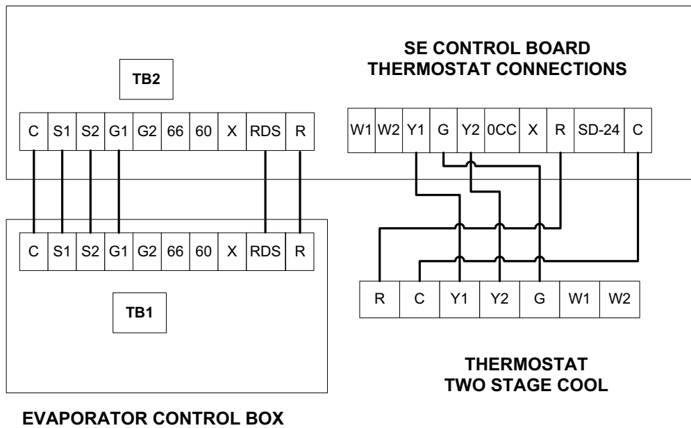
Figure 7: Typical field wiring diagram - GC300 evaporator unit with KC300 condenser unit
