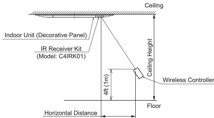
Horizontal Distance Limit for IR Receiver Kit (If the height of wireless controller from floor is 4 feet)
