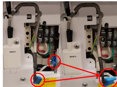
Figure 3 – Wi-Fi adapter installation
