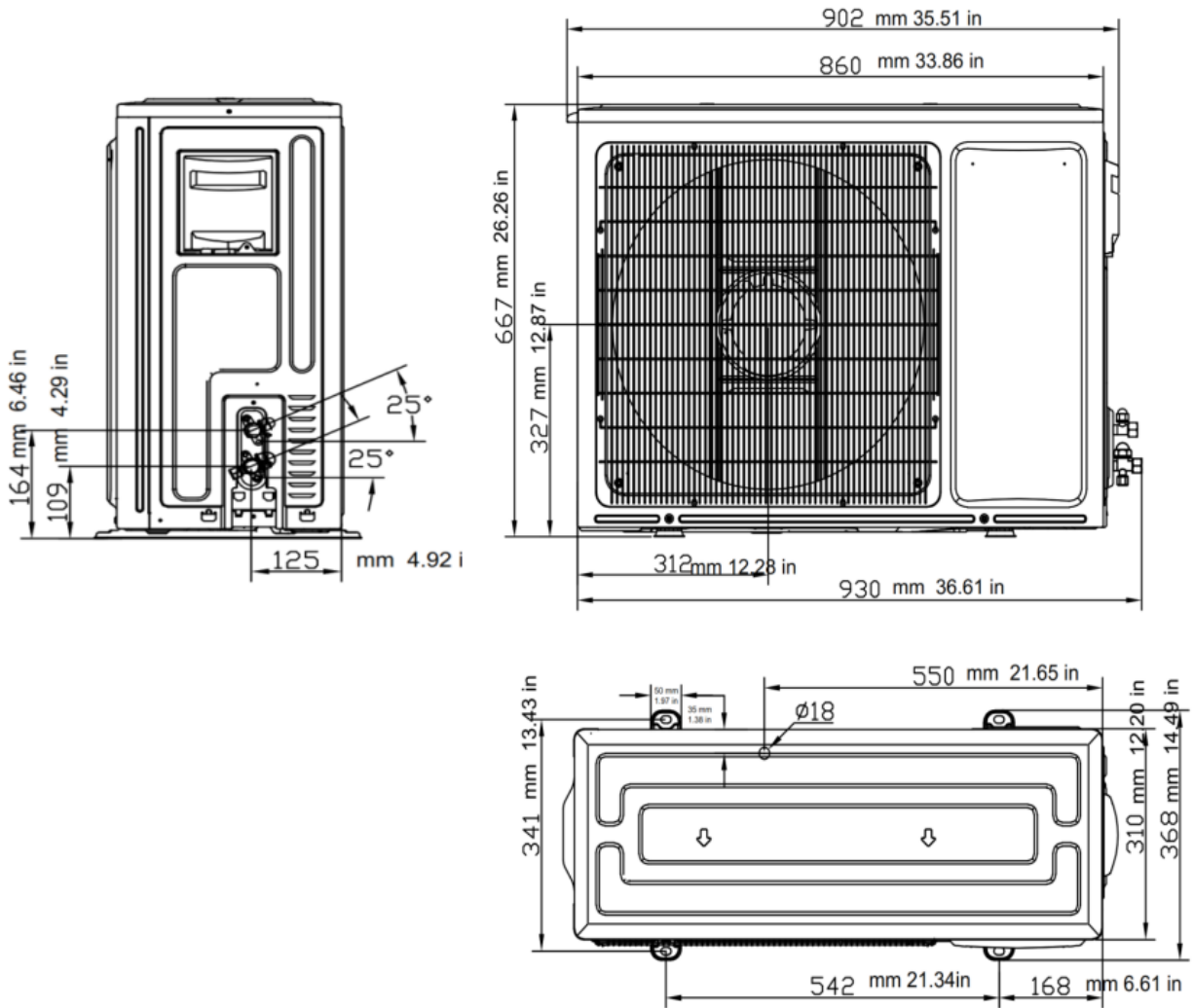
OUTDOOR UNIT
